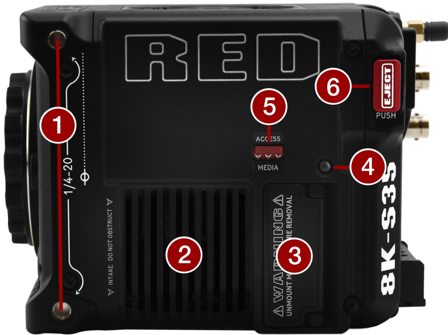
Figure: Camera Body Left Controls and Features
