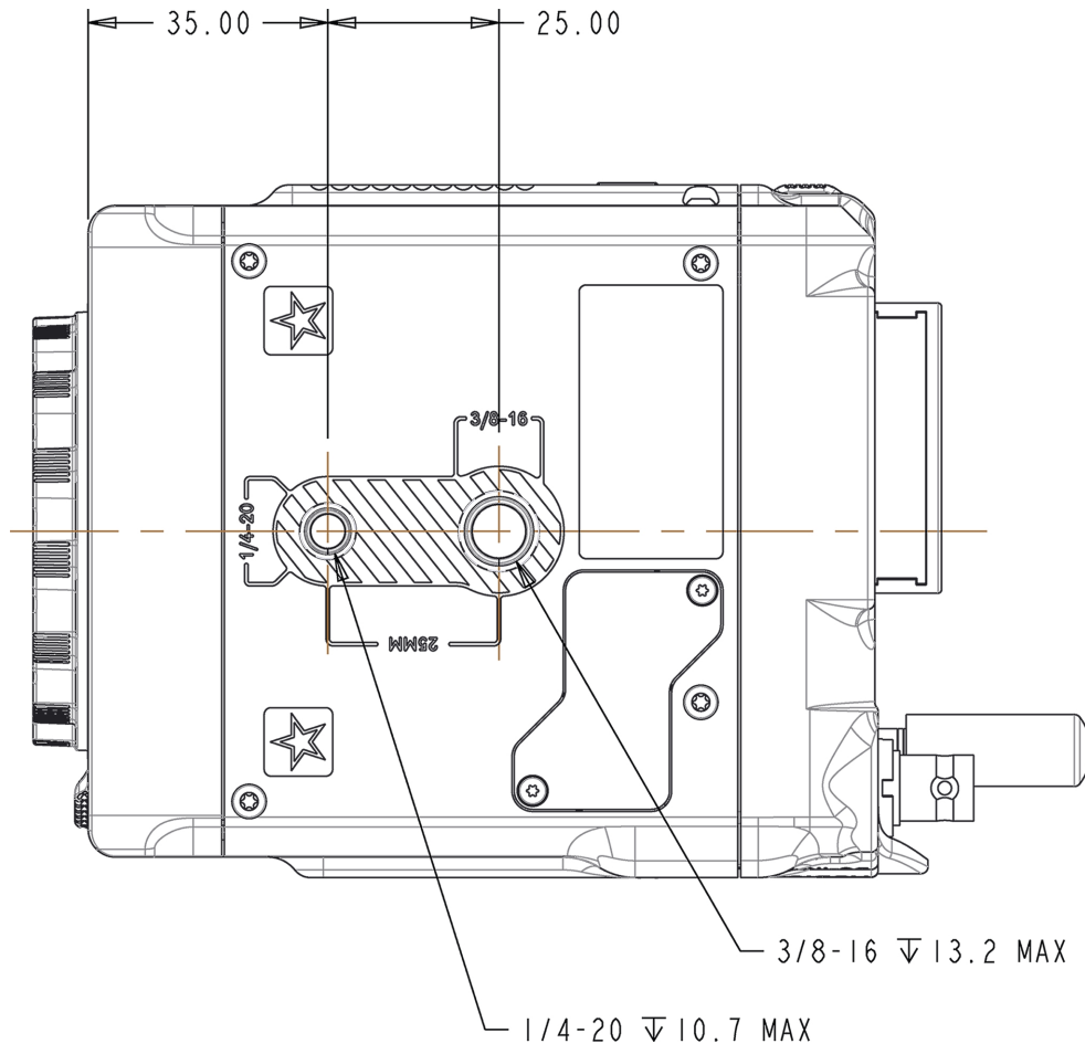
Figure: 摄像机底视图
