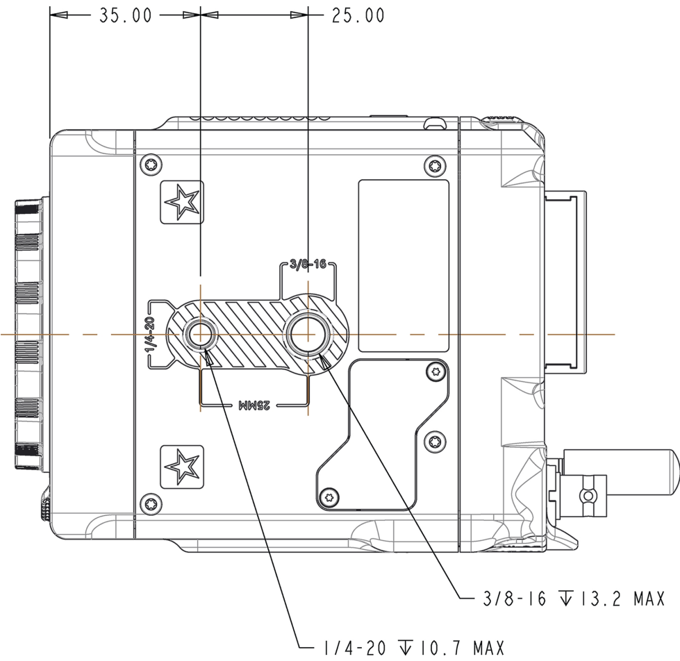
CF:图:相机底部视图, 射频
