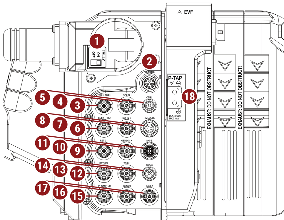
Figure: Module Right, Controls and Features
