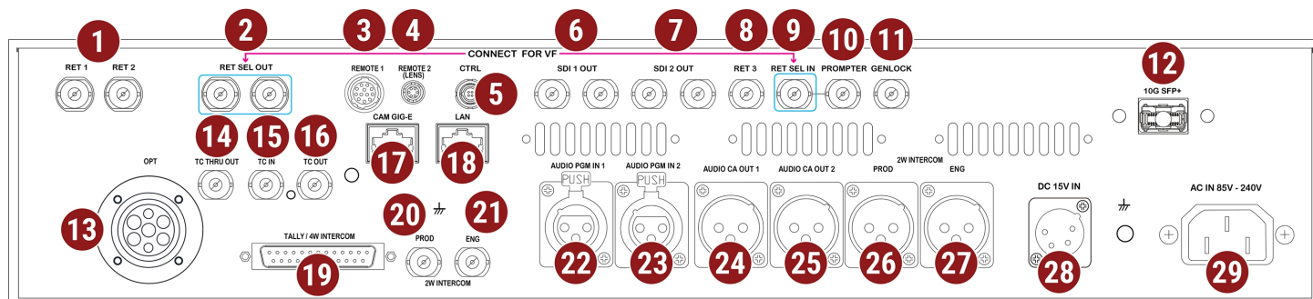
Figure: Base Station, ports
