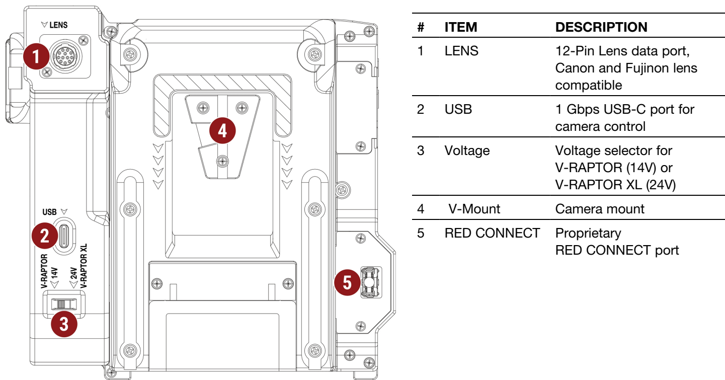
Figure: Module Front, Controls and Features
