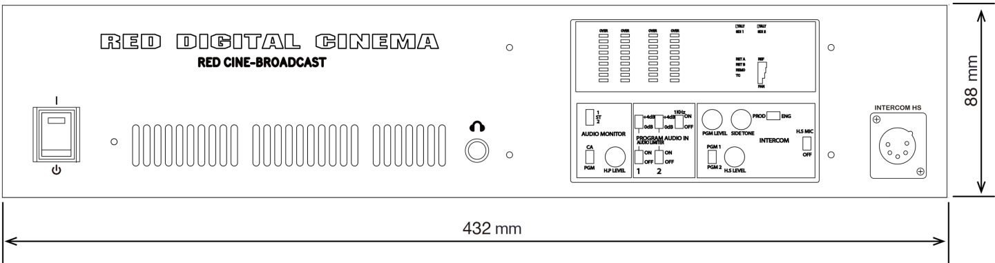
Figure: Base Station (Full Rack) Front View
