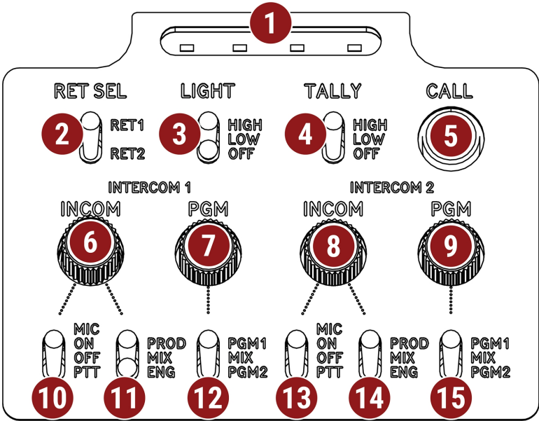
Figure: Back Panel, Controls and Features
