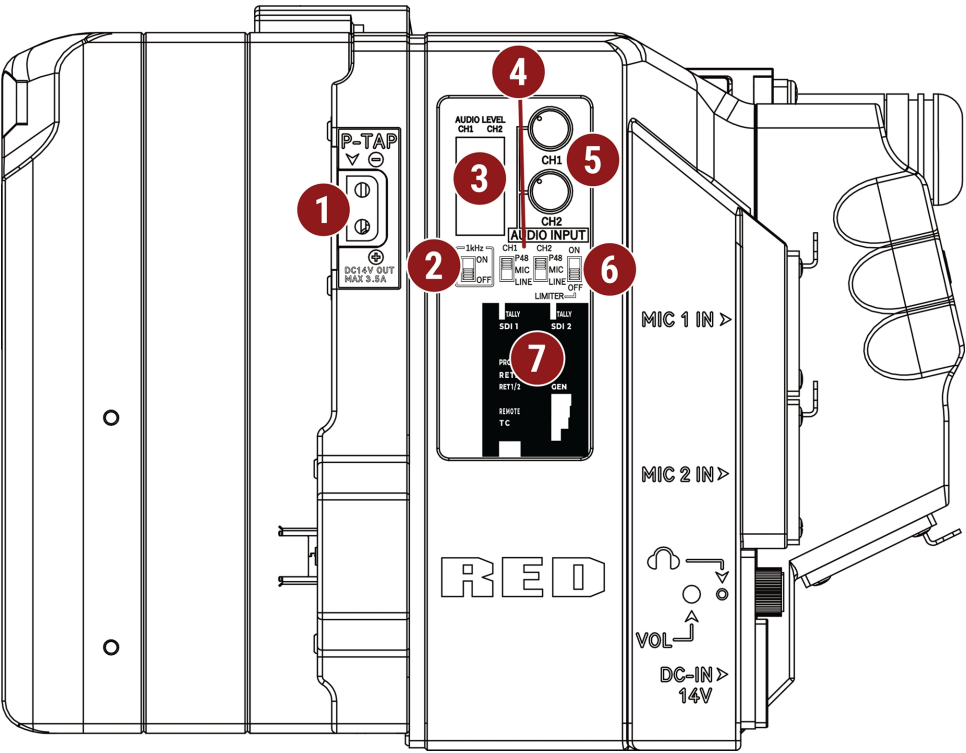
Figure: Module Left, Controls and Features
