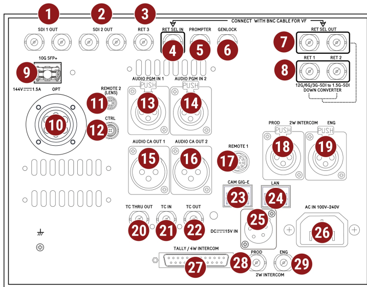
Figure: Half Rack Base Station Back, Controls and Features
