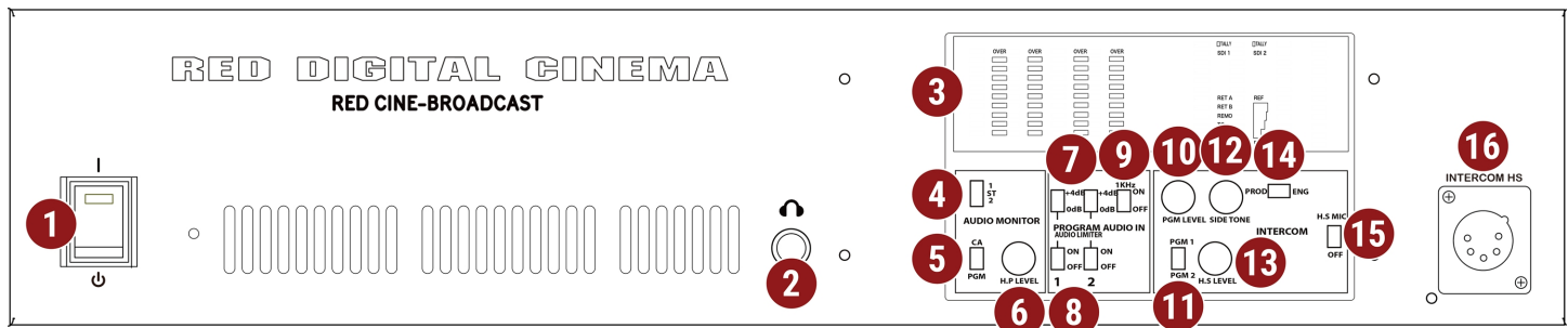
Figure: Base Station Front, Controls and Features
