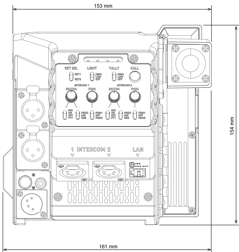
Figure: Module Rear View
