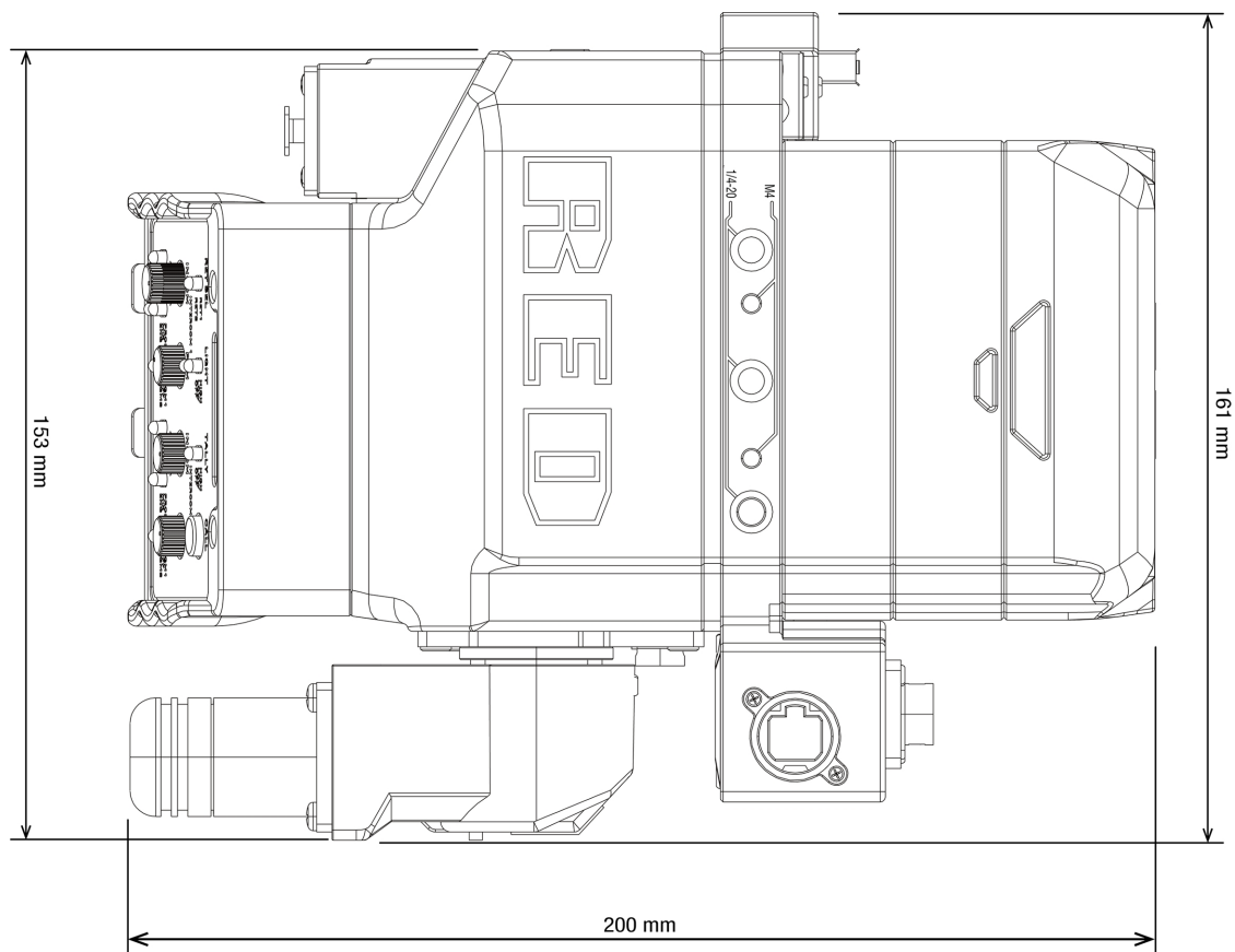
Figure: Module Top View
