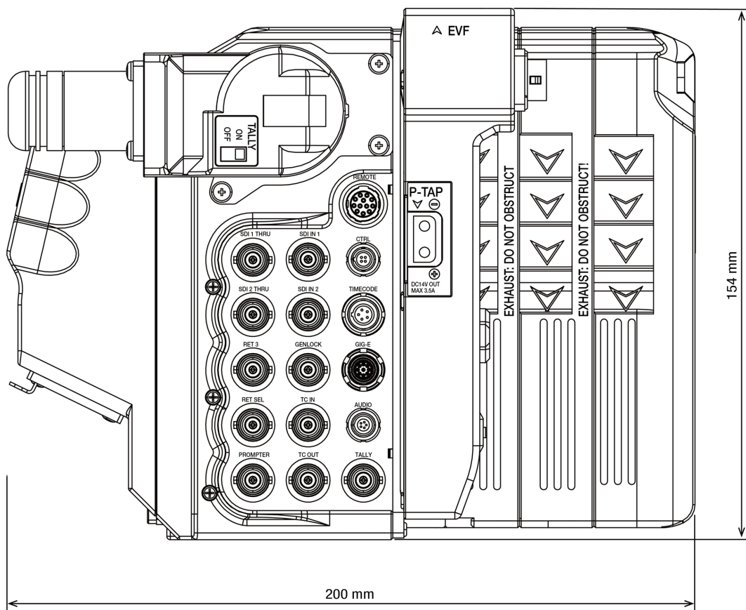
Figure: Module Side View (Right)
