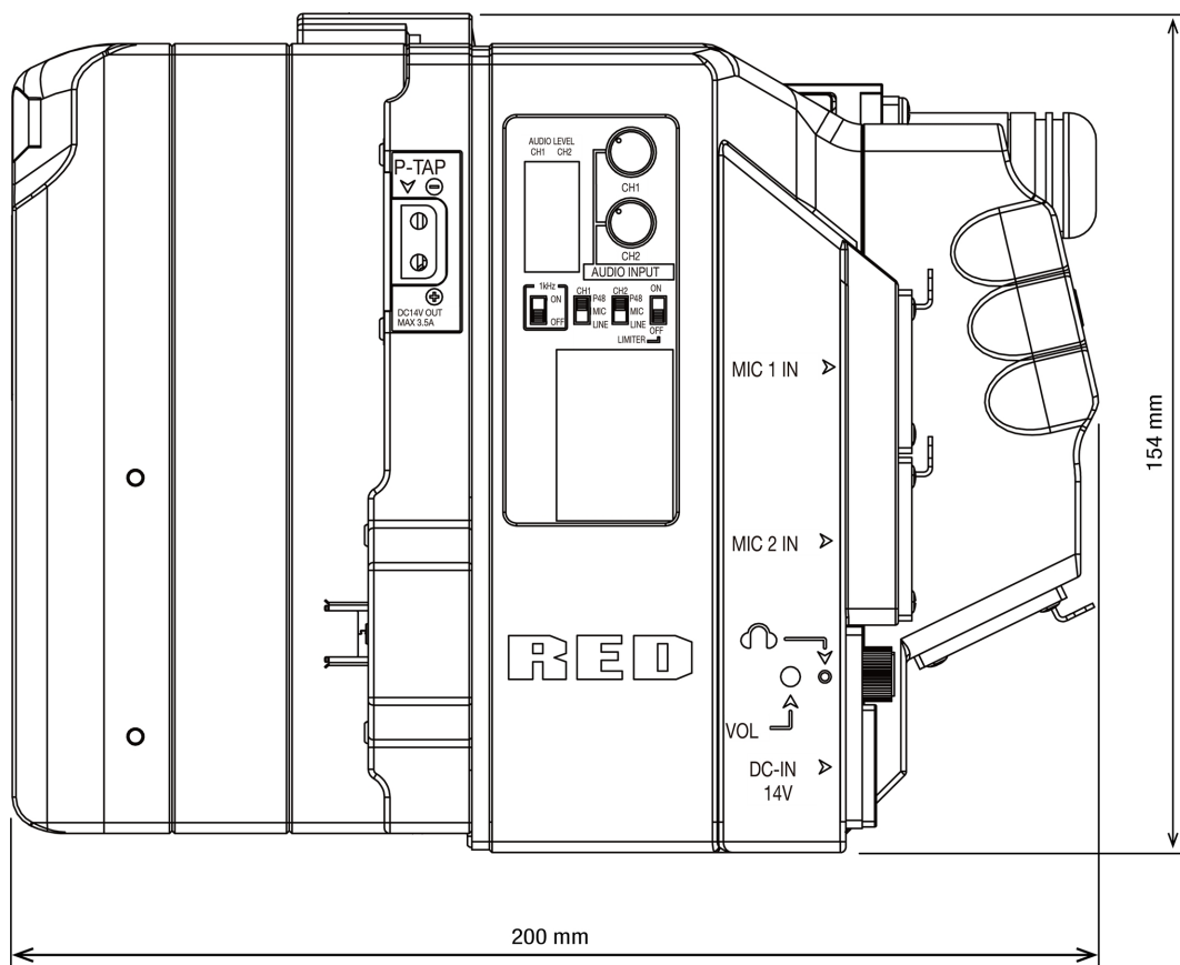
Figure: Module Side View (Left)
