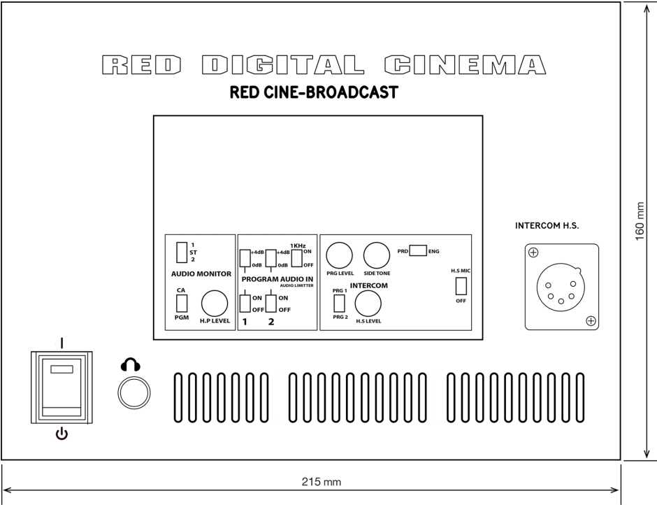
Figure: Base Station (Half Rack) Front View
