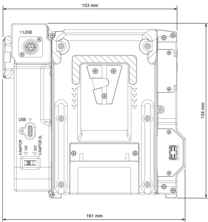
Figure: Module Front View
