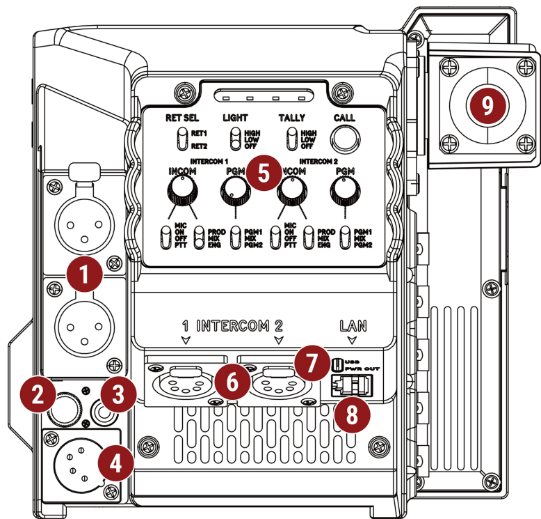
Figure: Module Rear, Controls and Features
