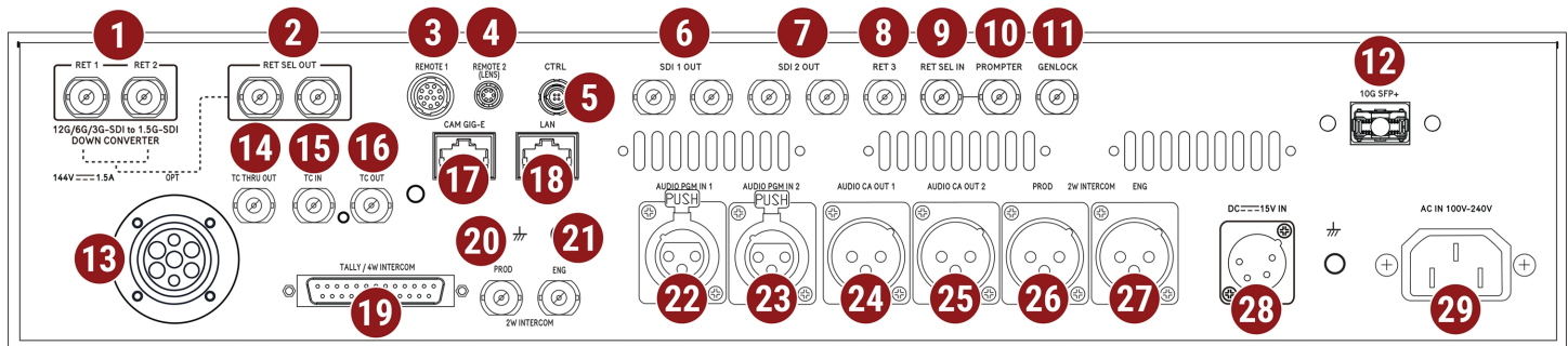
Figure: Base Station, ports
