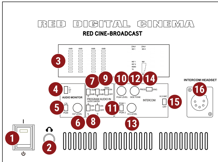
Figure: Half Rack Base Station Front, Controls and Features
