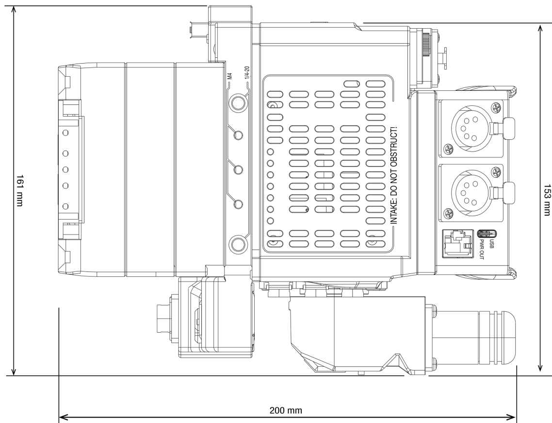
Figure: Module Bottom View
