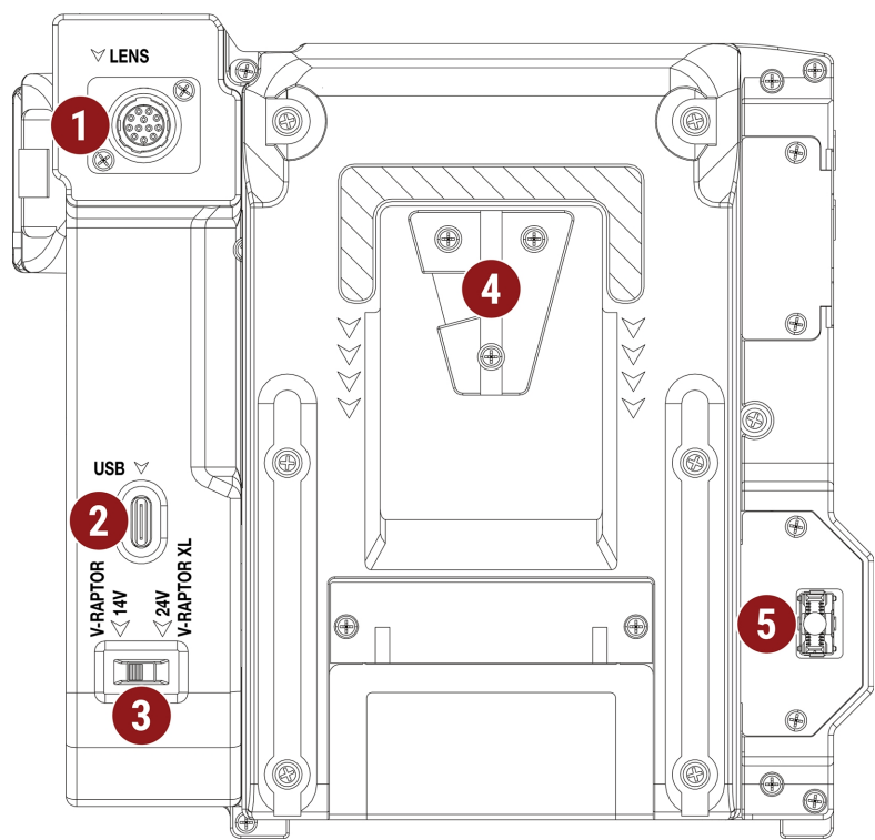
Figure: Module Front, Controls and Features
